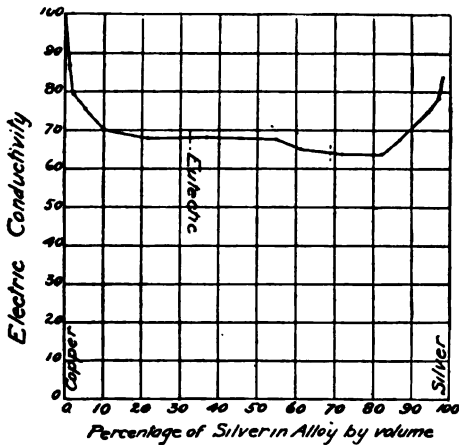
Fig. 56. Electric Conductivity Curve of Silver-copper Alloys.
